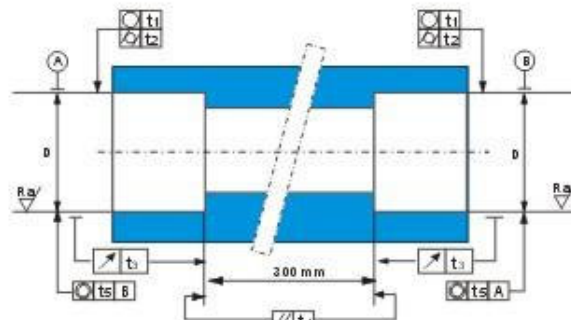
配合轴和座 Fitting shaft and housing
